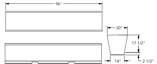
Details - ZB.WL.02
