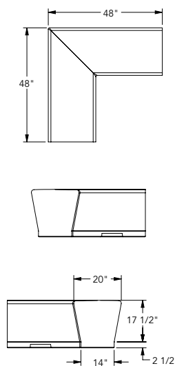
Details - ZB.WL.04
