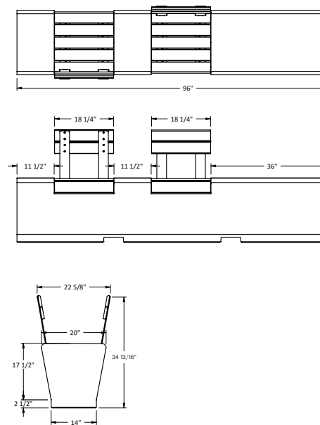
Details - ZB.WL.17
