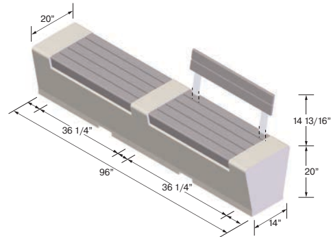
Details - ZB.WL.13
