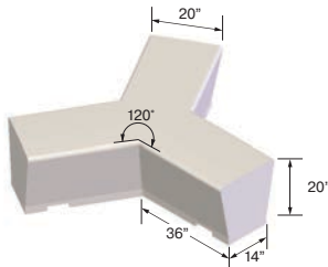
Details - ZB.WL.03
