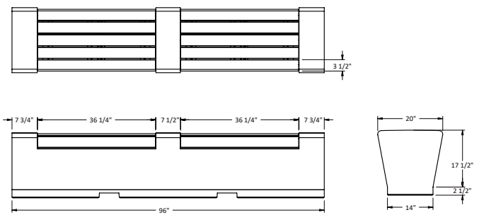
Details - ZB.WL.10
