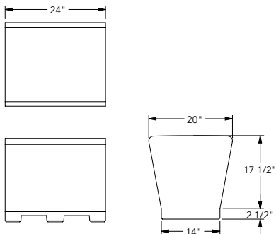
Details - ZB.WL.01
