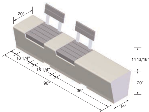
Details - ZB.WL.16
