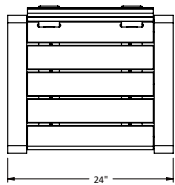
Details - ZB.WL.12
