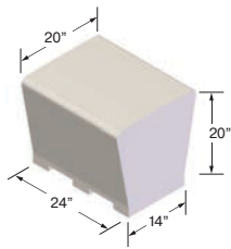
Details - ZB.WL.01
