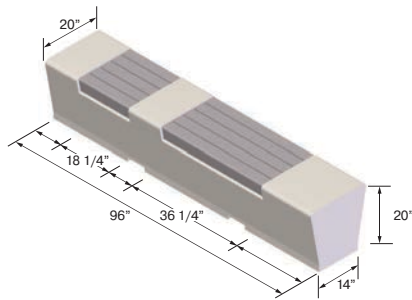
Details - ZB.WL.09
