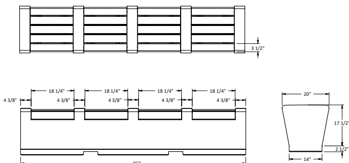
Details - ZB.WL.11
