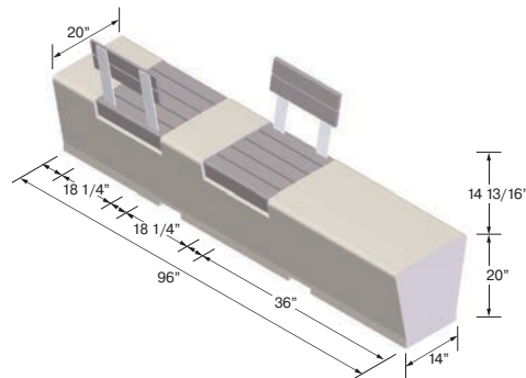
Details - ZB.WL.17
