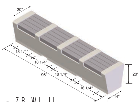
Details - ZB.WL.11
