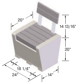
Details - ZB.WL.12
