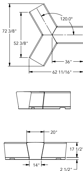
Details - ZB.WL.03
