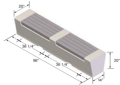
Details - ZB.WL.10
