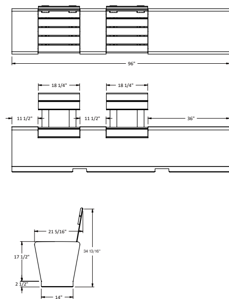
Details - ZB.WL.16
