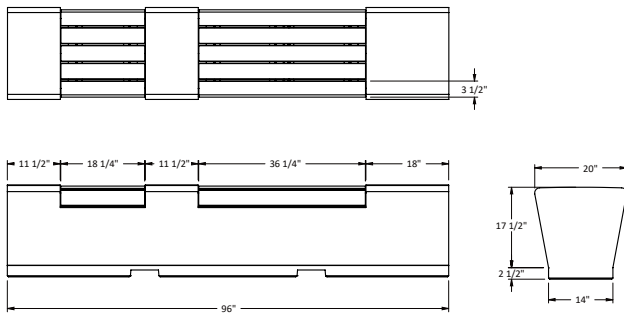
Details - ZB.WL.09
