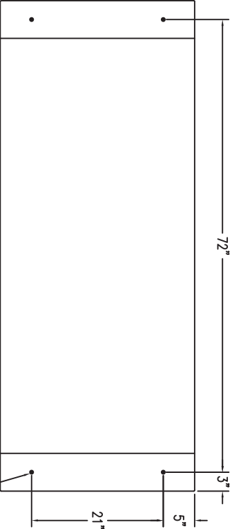
2 SIDE VIEW OF BENCH
